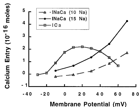
FIGURE 7 Calculated cellular Ca entry occurring via Ca current or reverse Na-Ca exchange alone. Calcium entry was calculated by integrating the first 150 ms of the whole-cell Ca currents recorded with no blockers present ( [Na]_p = 10 mM), or the nickel-sensitive currents recorded using the method shown in Fig. 5. Current integrals were converted to absolute [Ca^{2+}]_i 's, using Faraday's constant and the known charge movements during each type of current (see Results). Calcium entry by the two pathways is voltage dependent, and Na-Ca exchange is strongly influenced by [Na]_p .
