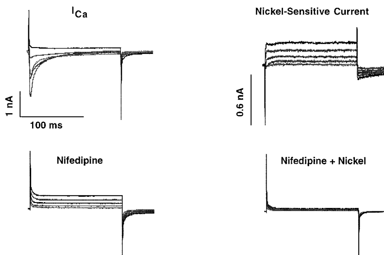
FIGURE 5 Measurement of putative Na-Ca exchange currents. In this representative example, the cell was voltage clamped with a pipette containing 15 mM Na. The cell was held at -40 mV. (A) The upper left panel shows Ca currents produced by voltage clamp steps between -30 and +70 mV (in 10-mV increments). (B) The cell was then exposed to 20 \mu\text{M} nifedipine, and the voltage clamp protocol was repeated. An outward current emerged when I_{\text{Ca}} was blocked. (C) Next, the cell was superfused with nifedipine and nickel (5 mM) (lower right). The outward current was reduced under these circumstances. (D) Finally, the currents in nickel plus nifedipine were subtracted from those in nifedipine alone. The nickel-sensitive difference current is probably due to reverse Na-Ca exchange.
